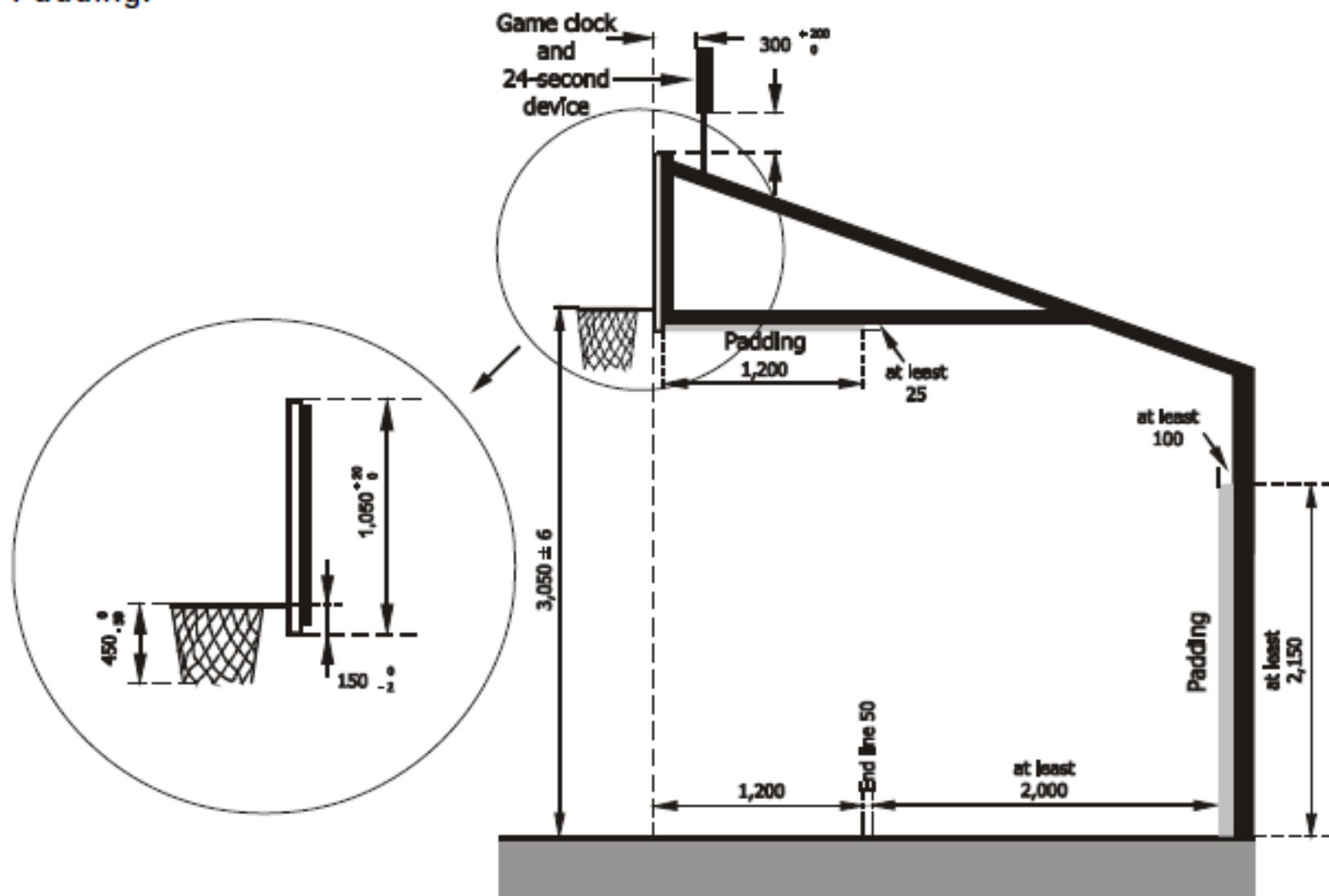
Diagram 1 Backstop unit
